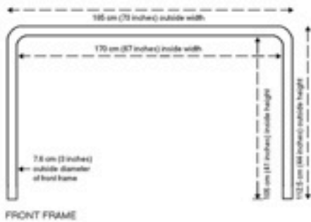
FRONT FRAME
