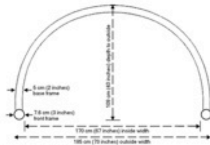
BASE STRUCTURE
